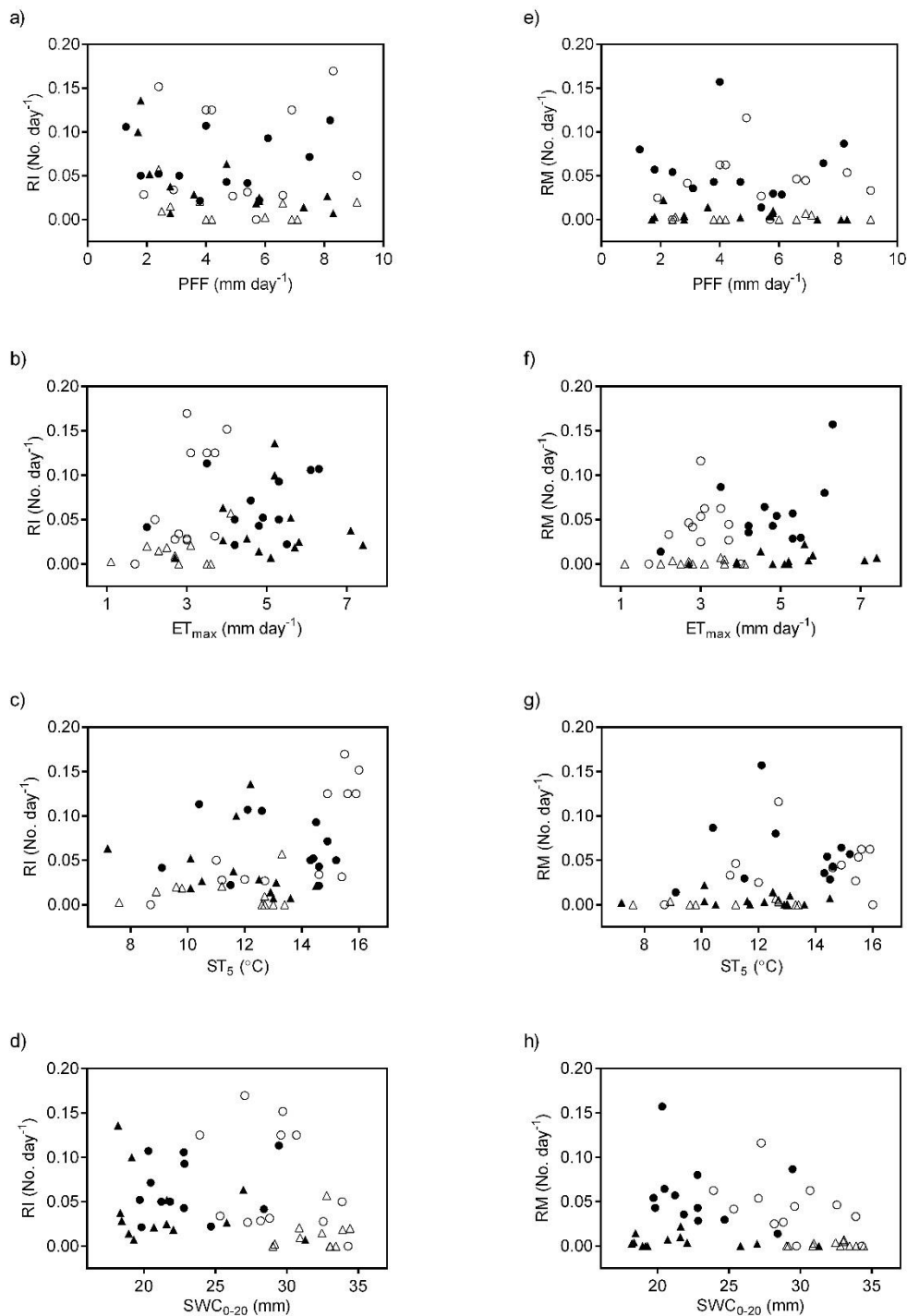
Figure 1. Relationships between fine root ingrowth ( RI ) ( \text{No. day}^{-1} ) and a) forest floor precipitation ( PFF ), b) maximum evapotranspiration ( ET_{max} , \text{mm day}^{-1} ), c) soil temperature at 5 cm depth ( ST_5 ), d) soil water content in 0-20 cm layer ( SWC_{0-20} , mm) and fine root mortality ( RM ) \text{No. day}^{-1} and e) forest floor precipitation ( PFF ), f) maximum evapotranspiration ( ET_{max} , \text{mm day}^{-1} ), g) soil temperature at 5 cm depth ( ST_5 ) and h) soil water content in 0-20 cm layer ( SWC_{0-20} , mm) for the two stands and gaps ( n=48 ). Triangles are for old-growth site and circles are for the managed site; open symbols indicate gap and filled symbols indicate stand.
